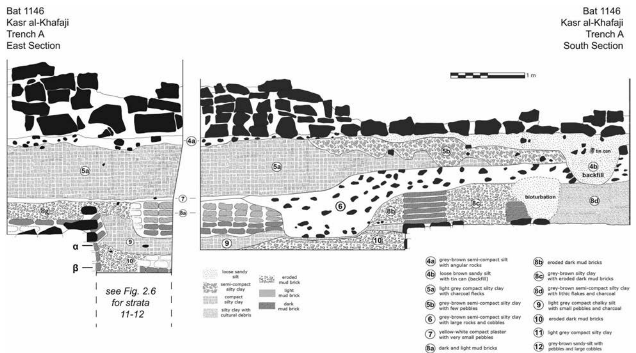
Figure 2.2. South and east sections of Trench A at Al-Khafaji tower showing the complex sequence of events from the Hafit walls at the bottom to the interior tower walls at the top (from Thornton 2016a: 40-41, fig. 3.17).
