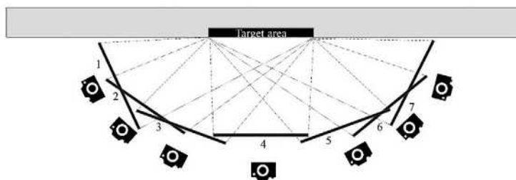
Figure 4. A simplified photogrammetric approach for SfM. Modified from Mol and Clarke, 2015.
