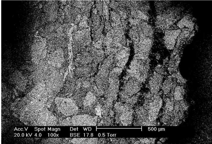
Figure 2. Scanning Electron Microscopy image of sandstone affected by ballistic impact, showing parallel fracturing at sub-surface level and associated loss of structural coherence of the stone. Image by the author.
